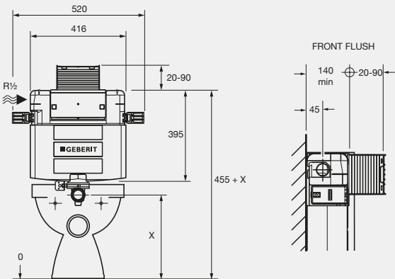
For Vanity/Hob - Top press 180mm, Front press 140mm
