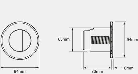
Sigma Round Dual-flush remote
