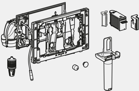
DuoFresh Odour Extraction Unit
