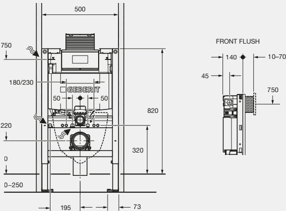
For Vanity/Hob - Top press 180mm, Front press 140mm
