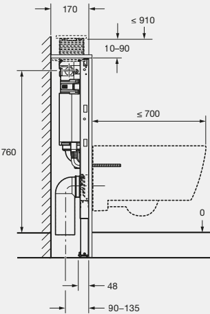
Omega Undercounter Cistern wall hung The Omega Undercounter cistern with frame is designed for mounting your wall hung pan into low height wall or hob wall installations. Geberit Omega Undercounter Cistern with frame Product Code: 30512
