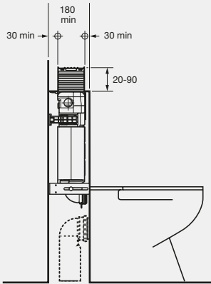
Omega Undercounter Cistern Back to wall The Omega Undercounter cistern back to wall is designed for floor mounted pans with low height wall or hob wall installations. Geberit Omega Undercounter Cistern Product Code: 1842017
