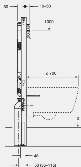
90mm wall cavity
